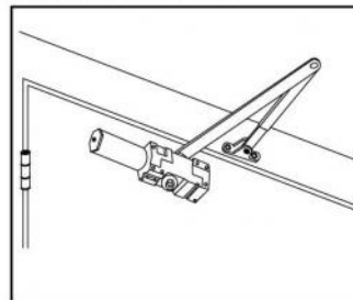
Regular Arm (Pull Side) Permit 120° maximum opening. See Page 2.
