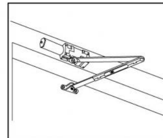
Top Jamb (Push Side) Permit 120° maximum opening. See Page 3.
